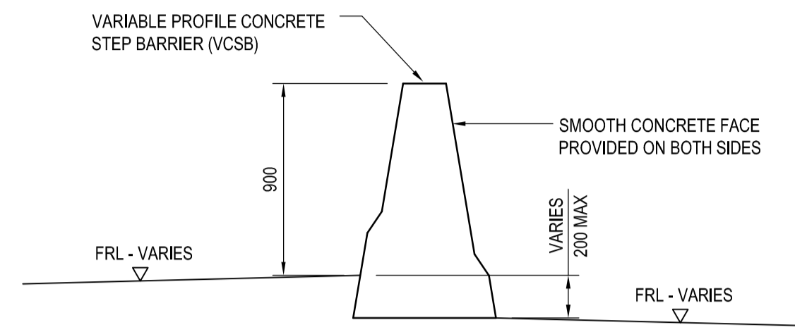
SECTION 1-1 (1:25)
